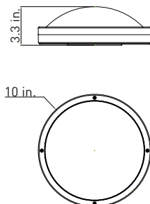
ROUND SHOREBREAKER LIGHT
