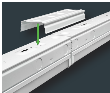
Joiner bracket snaps into place for 8 foot continuous mounting
