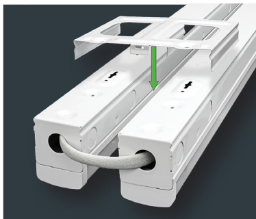
Brackets snap into place for parallel mounting
